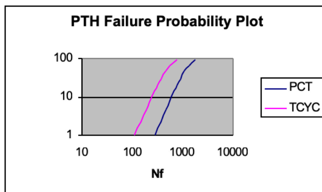
Figure 1: Calculated failure probability versus number of cycles for a 12-mil diameter PTH, 1.1-mil plated copper thickness, 0.125 inch thick PWB, T_g = 140^\circ\text{C} . PCT test is 25^\circ\text{C} to 130^\circ\text{C} at 96 cycles/day. TCYC test is -55^\circ\text{C} to 125^\circ\text{C} at 24 cycles/day.
