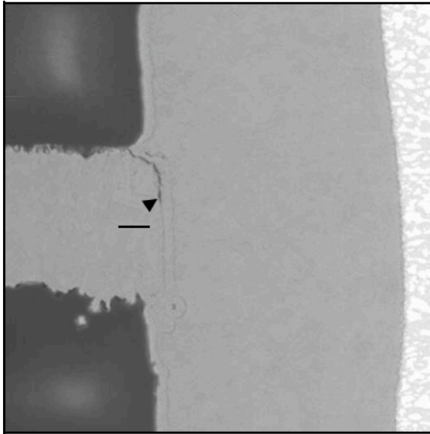
Figure 3: SEM image [810X] shows partial inner layer failure that was missed in conventional coupon evaluation (optical at 100X with 200X referee).
