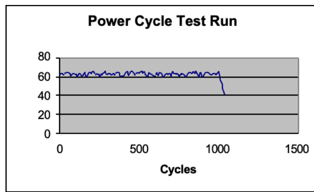
Figure 2: Power cycle test run showing heat-up time in seconds versus number of power cycles. The test circuit is typically heated from 25°C to 130°C and held at 130°C for a total power-on-cycle of 3 minutes (power-off-cycle is 12 minutes).
