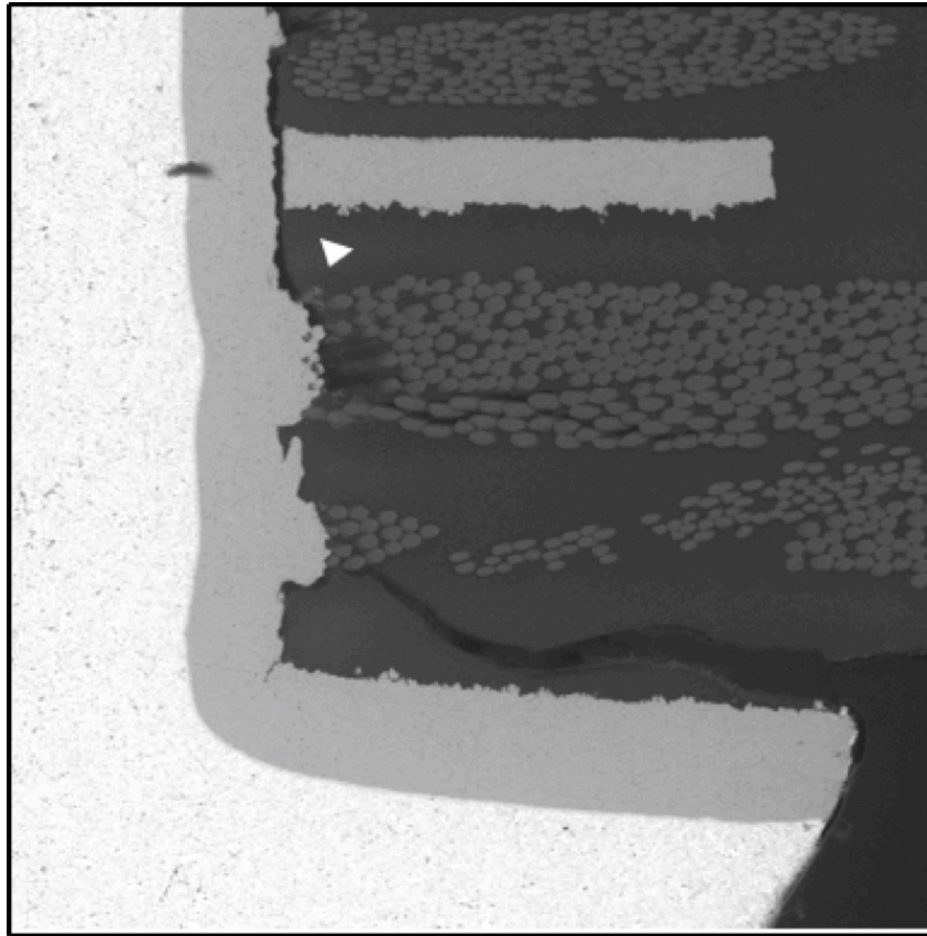
Figure 4: SEM image [162X] shows section of a failed PTH (field failure) due to inner layer separation.
